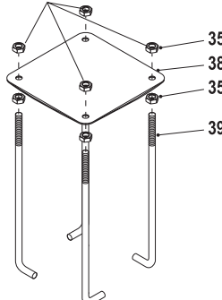
Detail A Bottom View
